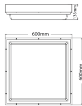
Surface Mounting
