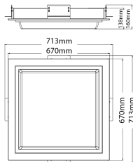
Recessed Mounting
